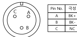
&lt;Brake Connector&gt;
