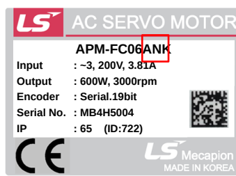
Absolute Singleturn(절대치싱글턴)
