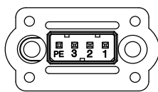
&lt;Power Connector 핀 배열&gt;
