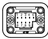
&lt;Encoder Connector 핀 배열&gt;
