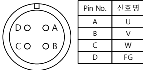
&lt;Power Connector&gt;
