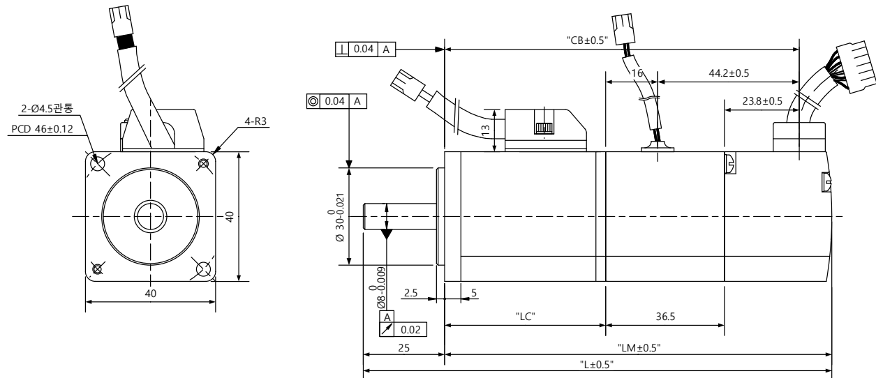
&lt;Power Connector&gt;
