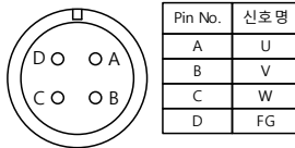
&lt;Power Connector&gt;
