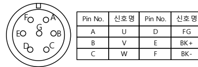
&lt;Brake Type Connector&gt;
