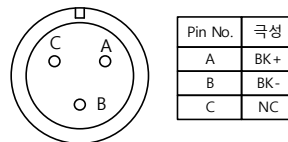
&lt;Brake Connector&gt;
